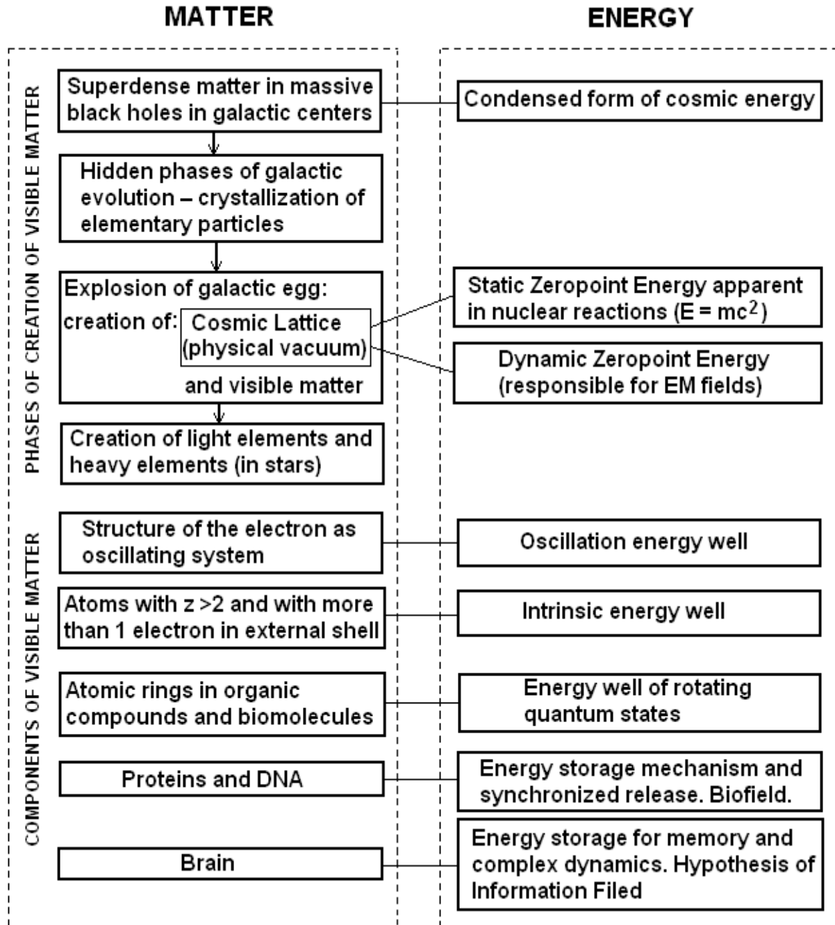
Fig. 6. Matter – energy diagram according to the BSM – Supergravitation Unified Theory
