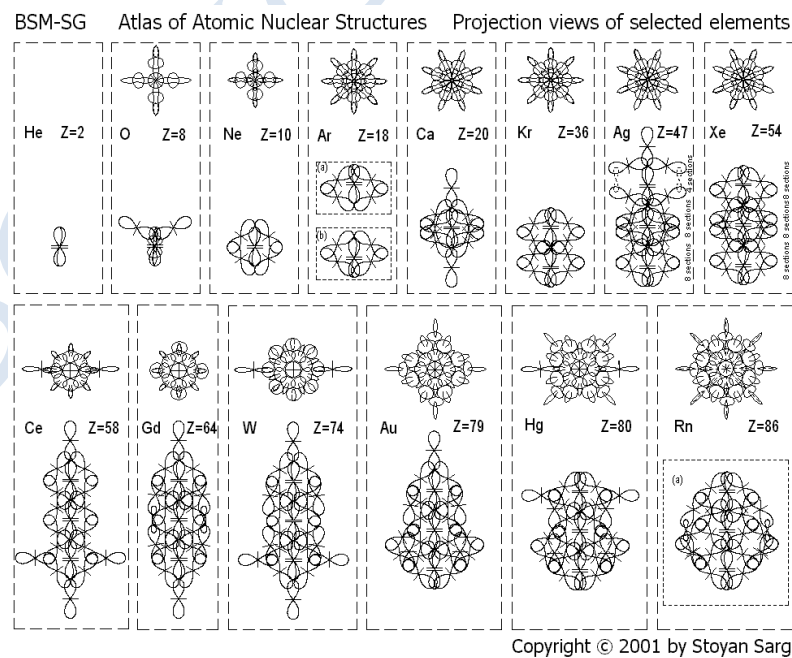
Fig. 2. Atomic nuclei of some selected elements
